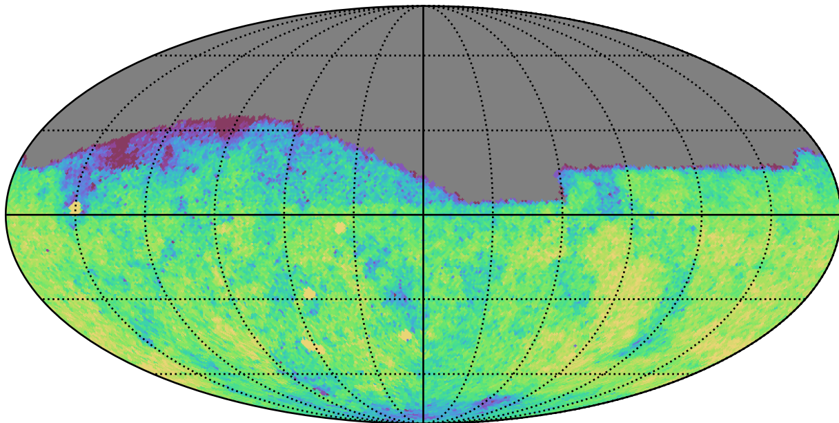
weather_cloudso20v3.4_10yrs Yr 1 g band: CoaddM5
