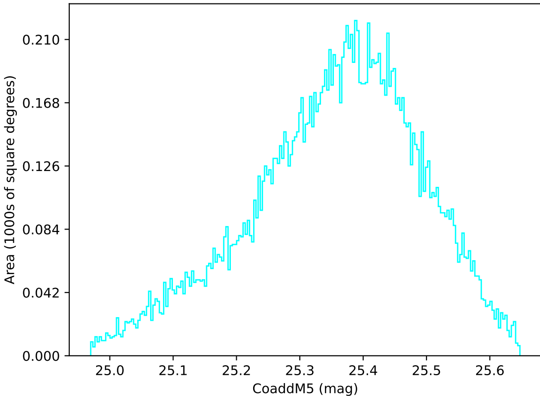
weather_cloudso20v3.4_10yrs WFD u band: CoaddM5
