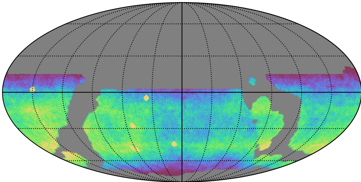
weather_cloudso20v3.4_10yrs WFD r band: CoaddM5
