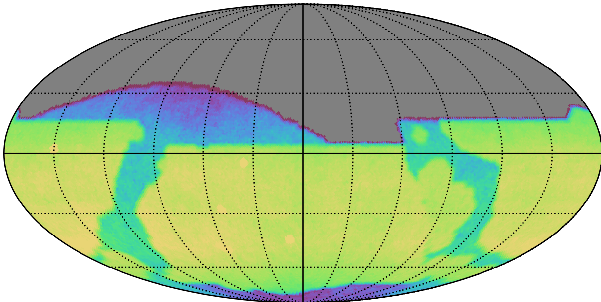
weather_cloudso20v3.4_10yrs All sky z band: CoaddM5
