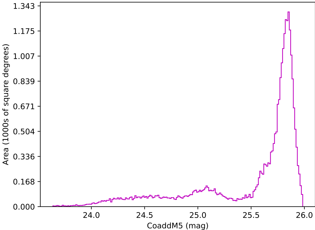
weather_cloudso20v3.4_10yrs All sky z band: CoaddM5
