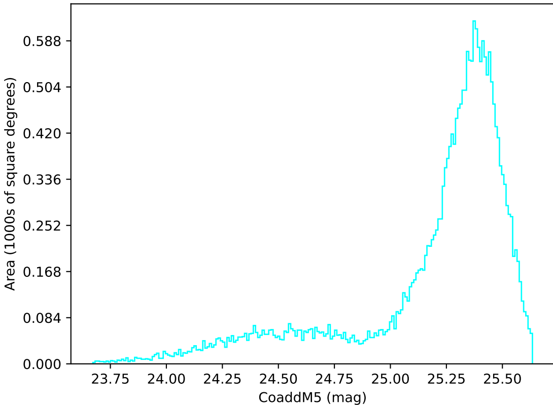
weather_cloudso20v3.4_10yrs All sky u band: CoaddM5
