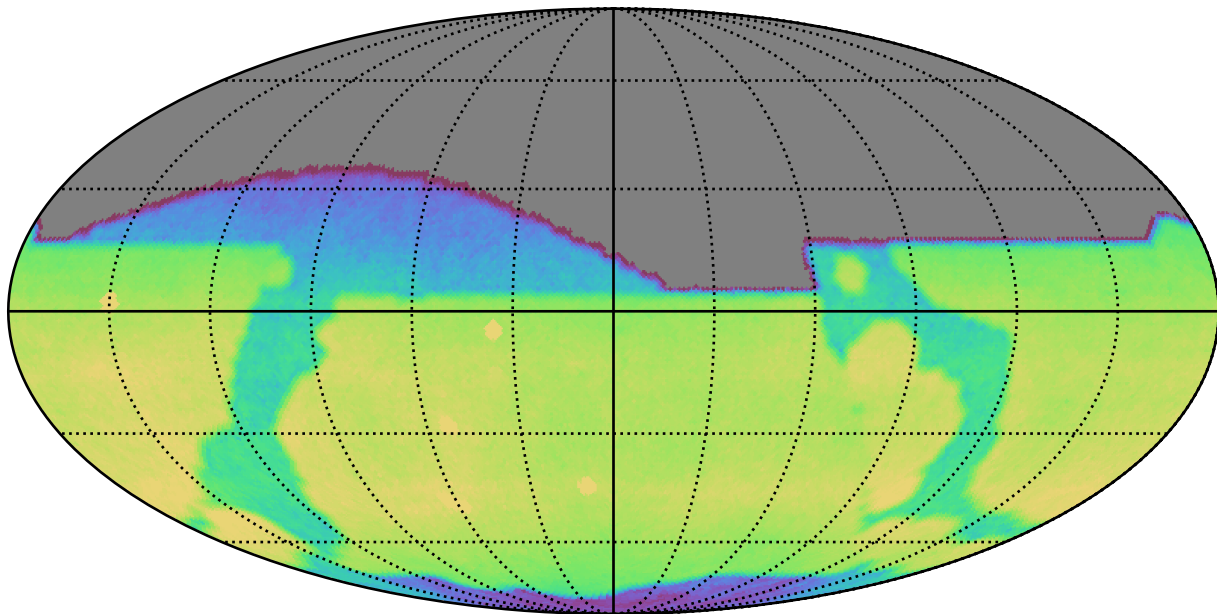
weather_cloudso20v3.4_10yrs All sky r band: CoaddM5
