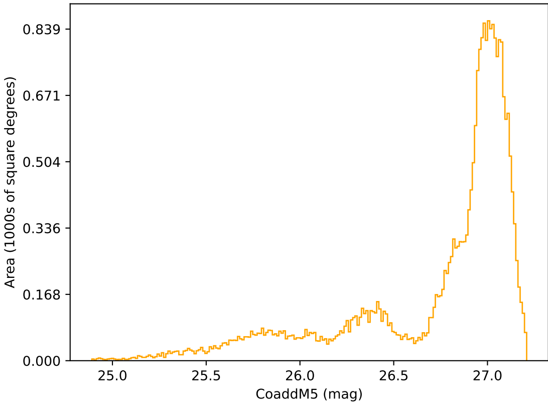
weather_cloudso20v3.4_10yrs All sky r band: CoaddM5
