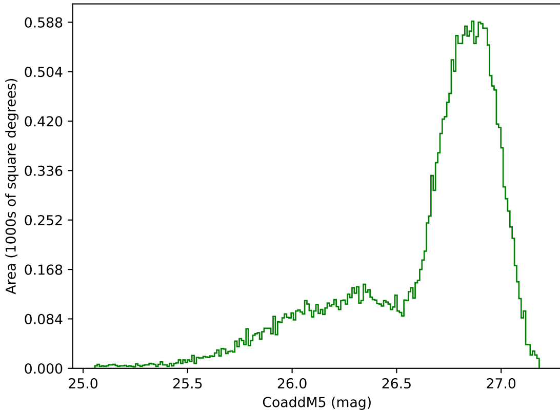
weather_cloudso20v3.4_10yrs All sky g band: CoaddM5
