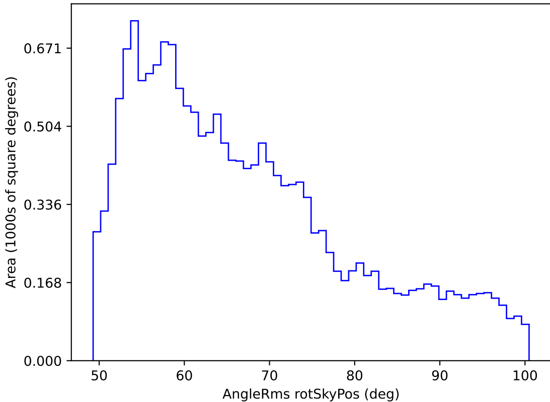
weather_cloudso20v3.4_10yrs WFD all bands: AngleRms rotSkyPos
