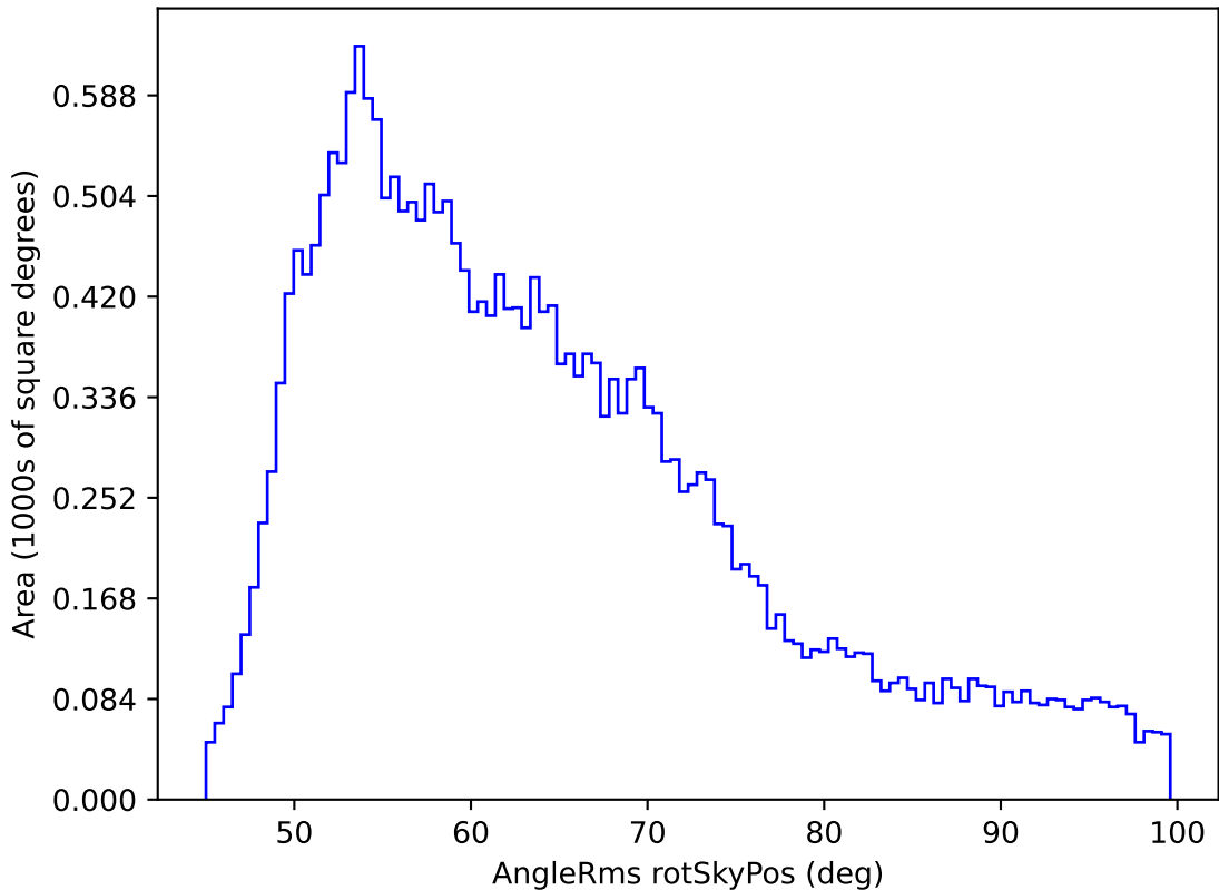
weather_cloudso20v3.4_10yrs All sky all bands: AngleRms rotSkyPos
