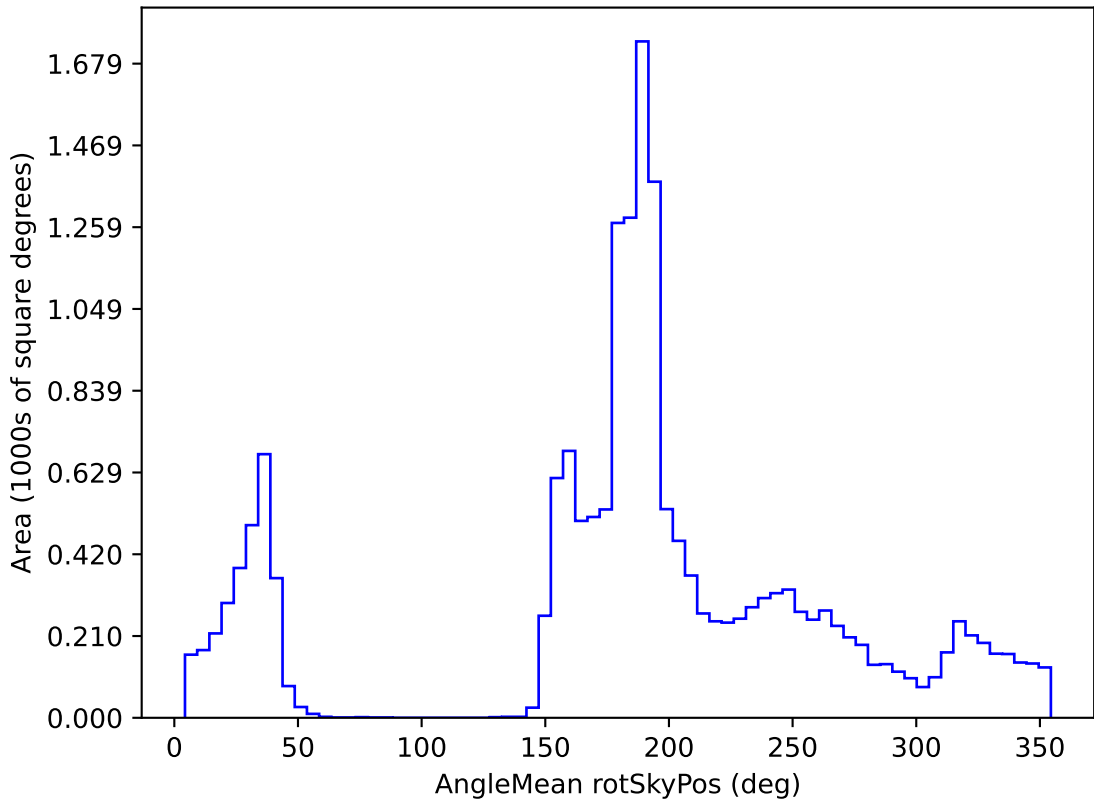
weather_cloudso20v3.4_10yrs WFD all bands: AngleMean rotSkyPos
