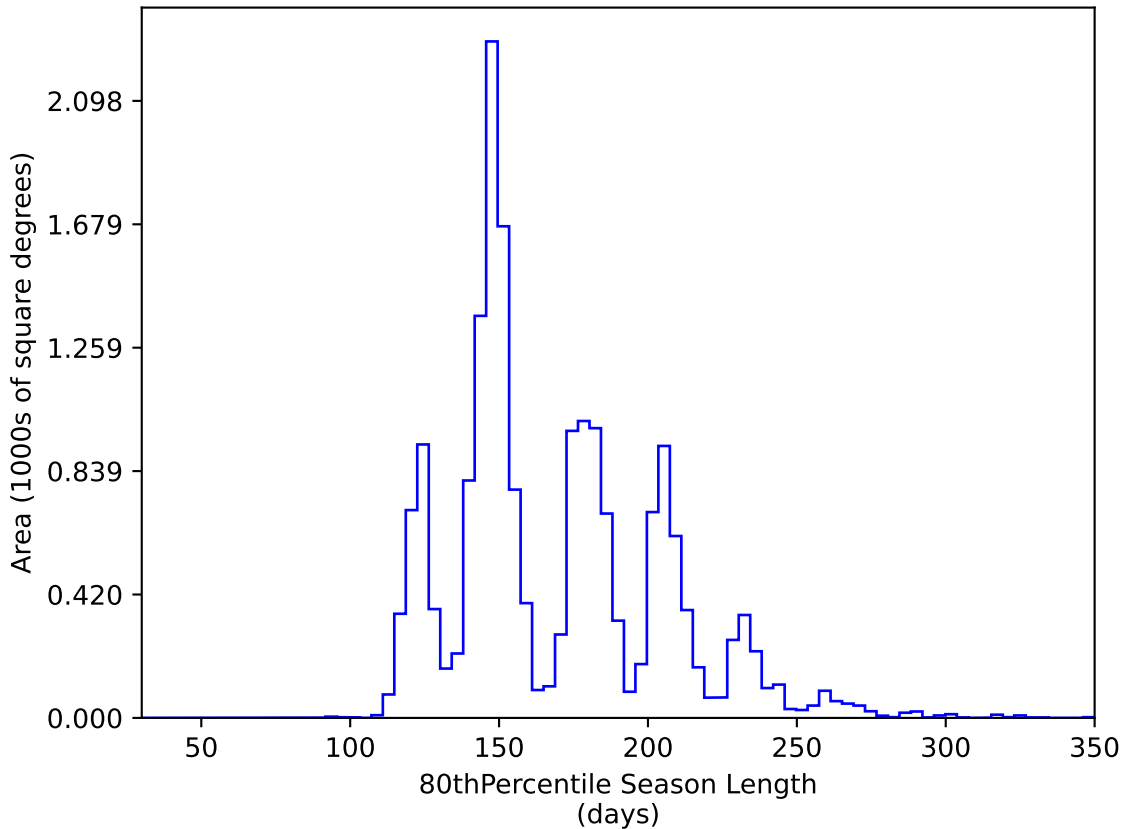
weather_cloudso20v3.4_10yrs WFD y band: 80thPercentile Season Length
