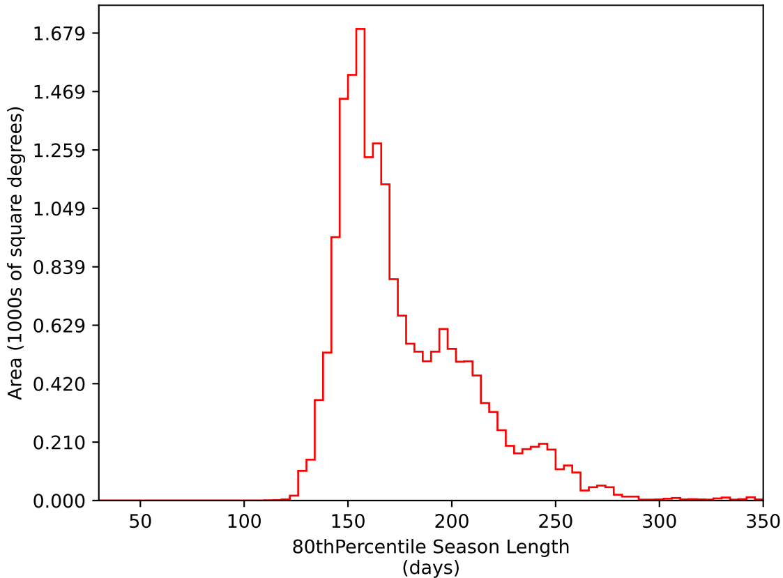
weather_cloudso20v3.4_10yrs WFD i band: 80thPercentile Season Length
