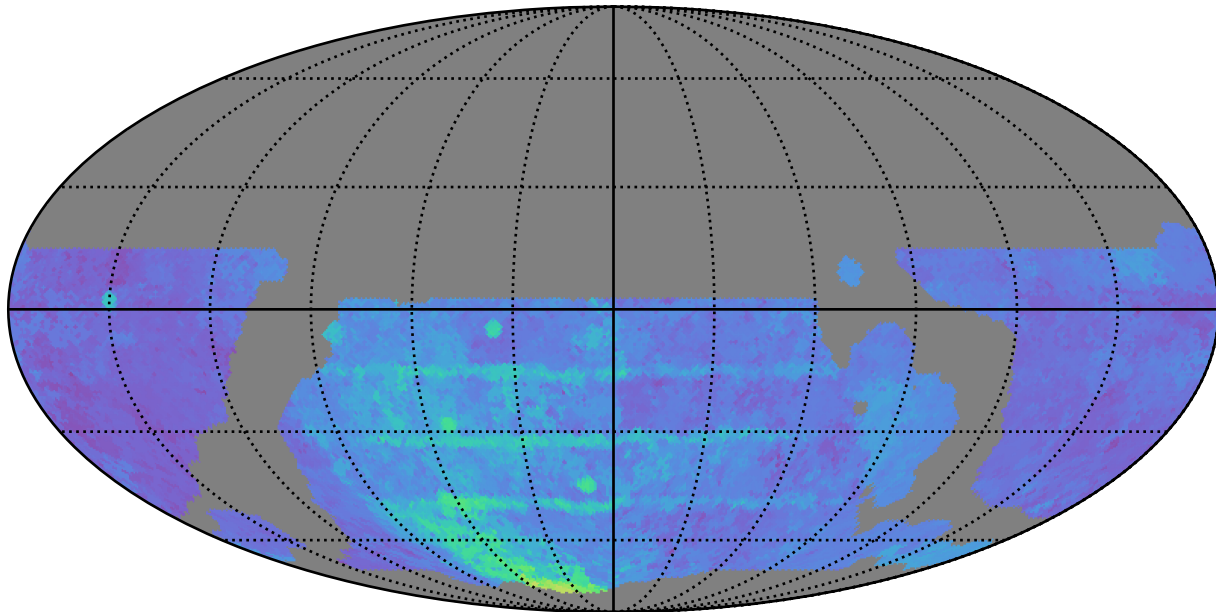
weather_cloudso20v3.4_10yrs WFD g band: 80thPercentile Season Length
