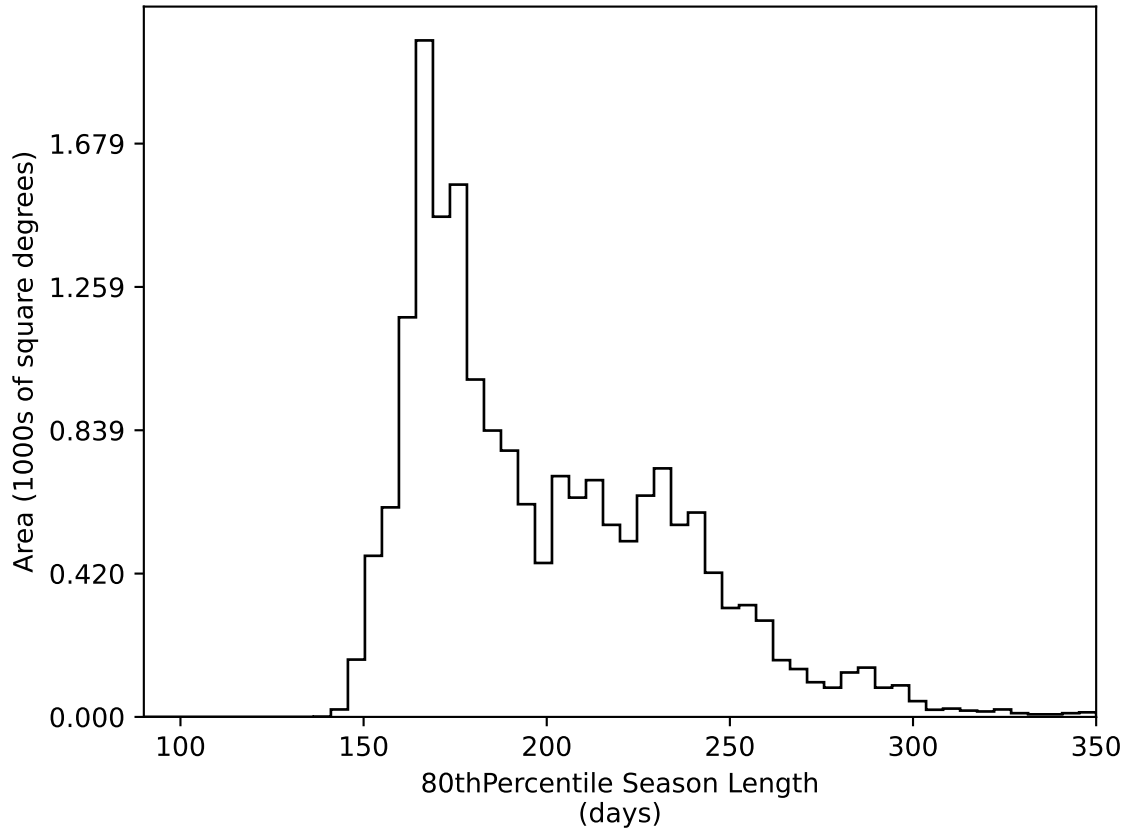
weather_cloudso20v3.4_10yrs WFD all bands: 80thPercentile Season Length
