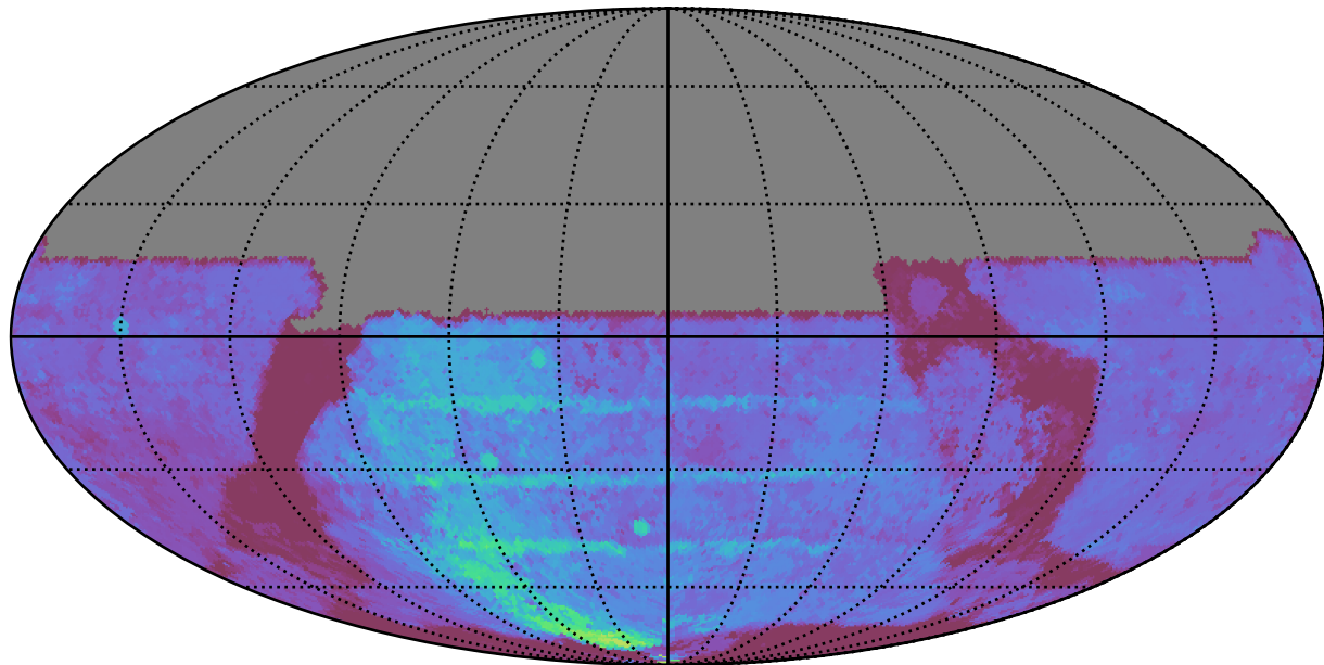
weather_cloudso20v3.4_10yrs All sky u band: 80thPercentile Season Length
