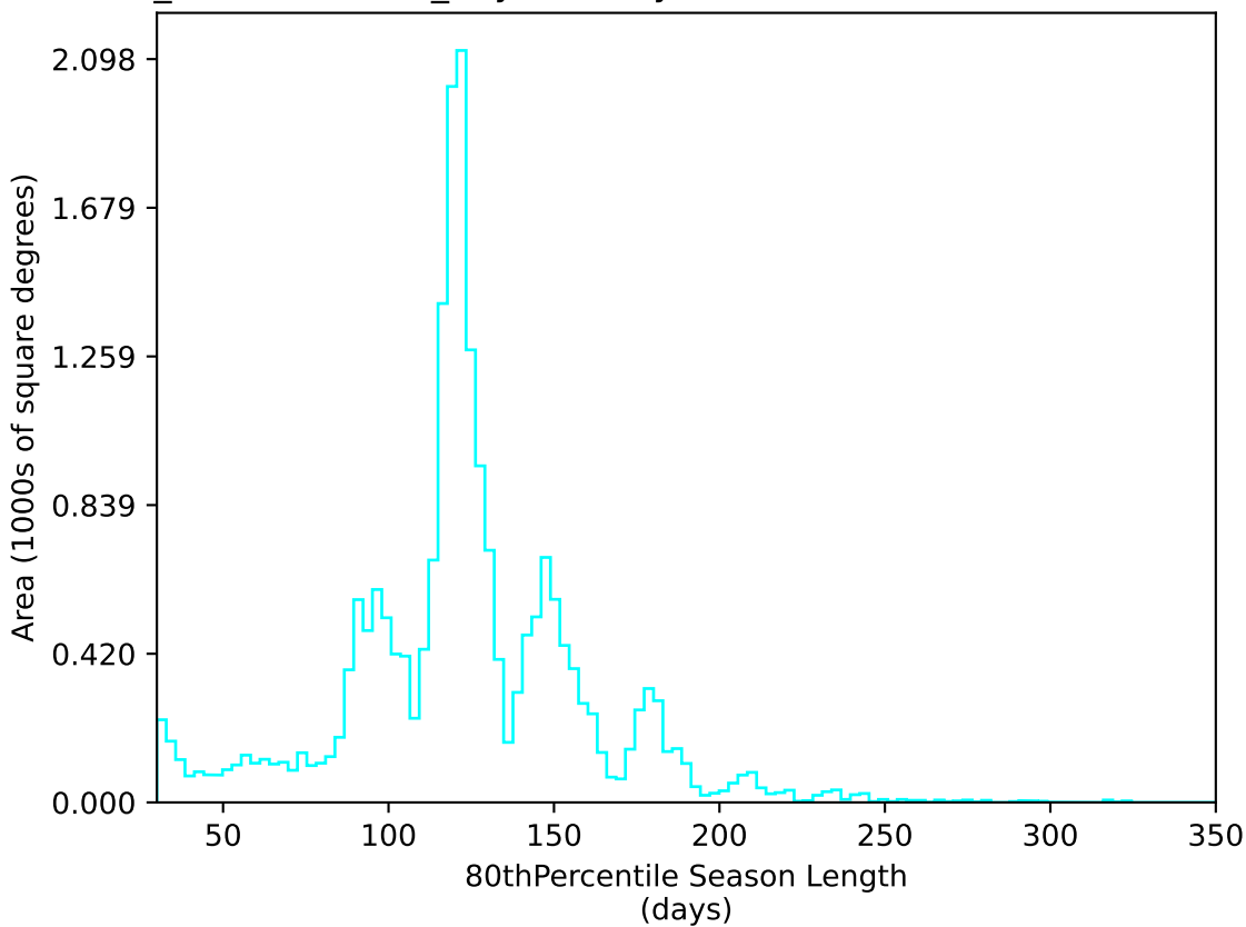
weather_cloudso20v3.4_10yrs All sky u band: 80thPercentile Season Length
