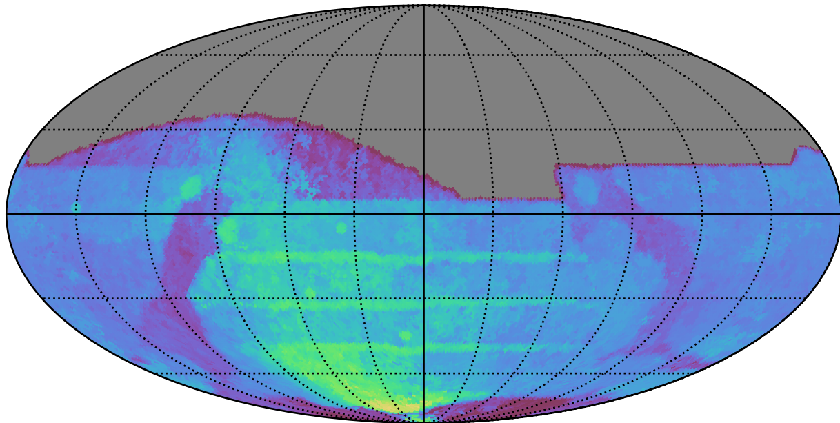
weather_cloudso20v3.4_10yrs All sky r band: 80thPercentile Season Length
