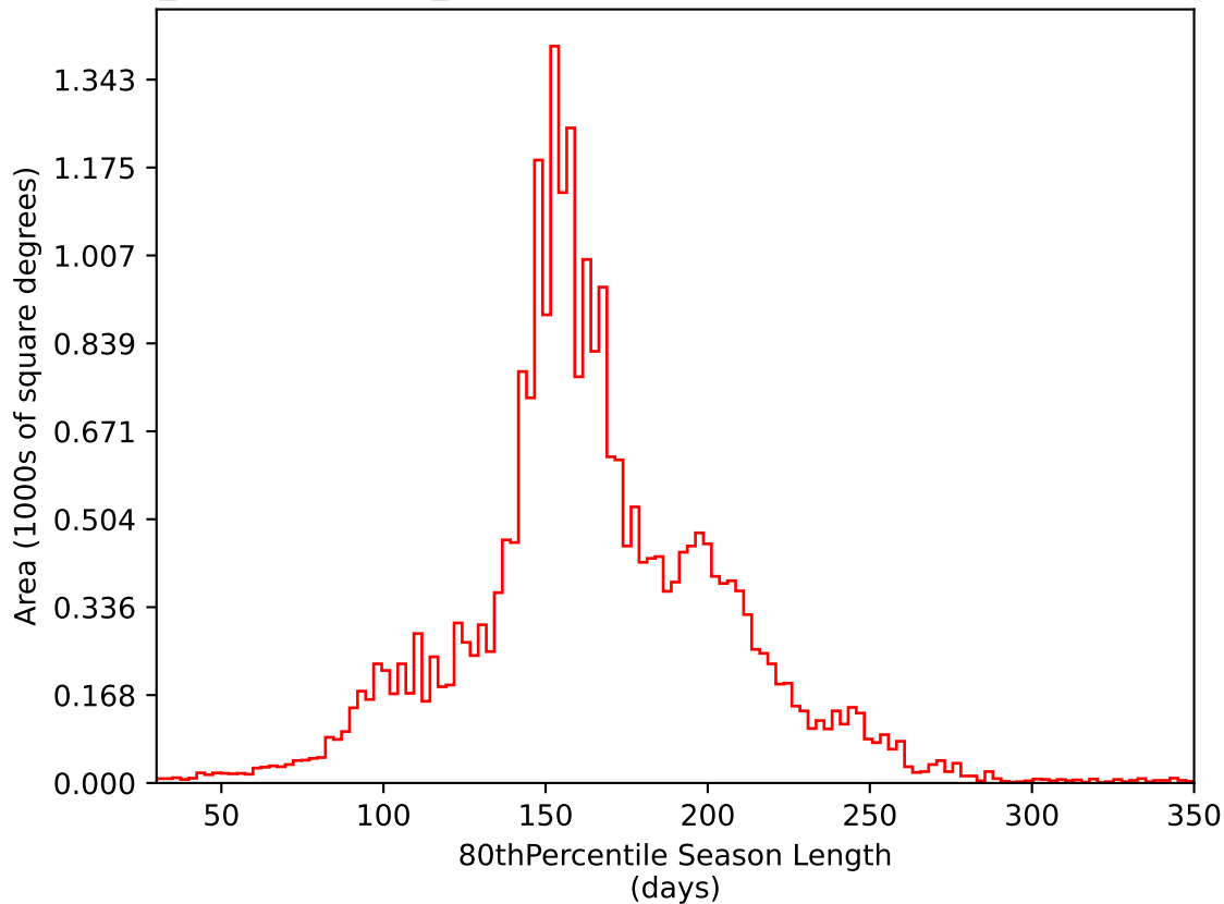
weather_cloudso20v3.4_10yrs All sky i band: 80thPercentile Season Length
