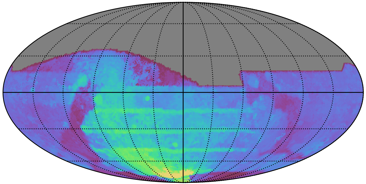
weather_cloudso20v3.4_10yrs All sky all bands: 80thPercentile Season Length
