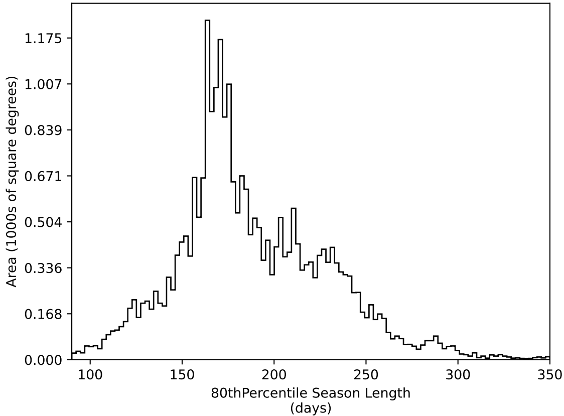
weather_cloudso20v3.4_10yrs All sky all bands: 80thPercentile Season Length
