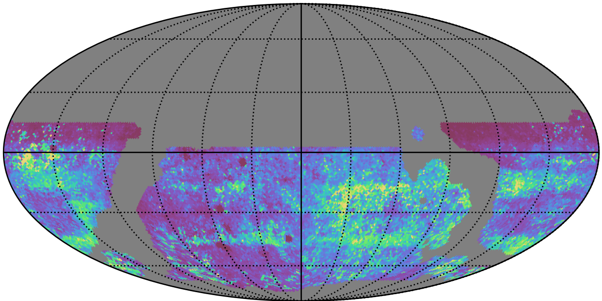
weather_cloudso20v3.4_10yrs WFD zy bands: 75th Percentile Intranight Timespan
