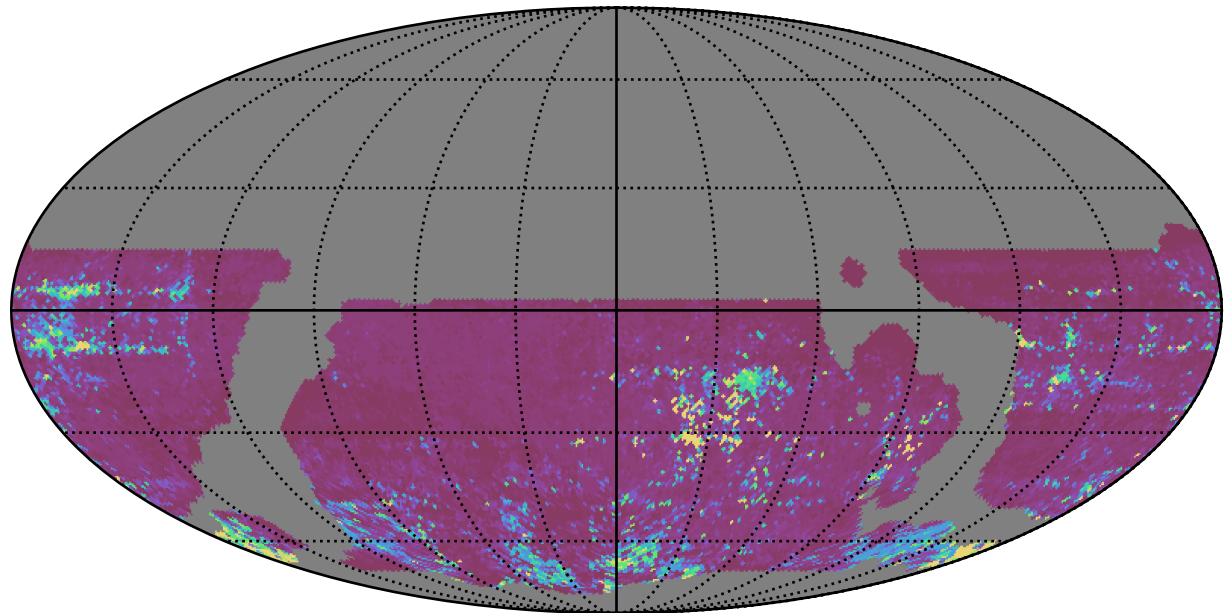
weather_cloudso20v3.4_10yrs WFD z band: 75th Percentile Intranight Timespan
