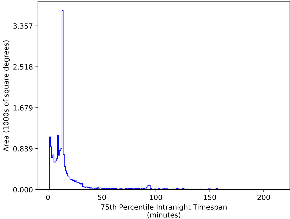
weather_cloudso20v3.4_10yrs WFD z band: 75th Percentile Intranight Timespan
