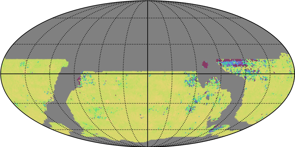
weather_cloudso20v3.4_10yrs WFD ug bands: 75th Percentile Intranight Timespan
