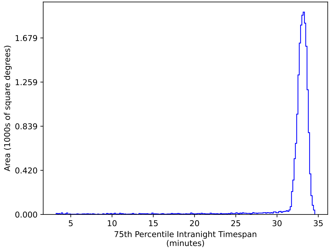
weather_cloudso20v3.4_10yrs WFD ug bands: 75th Percentile Intranight Timespan
