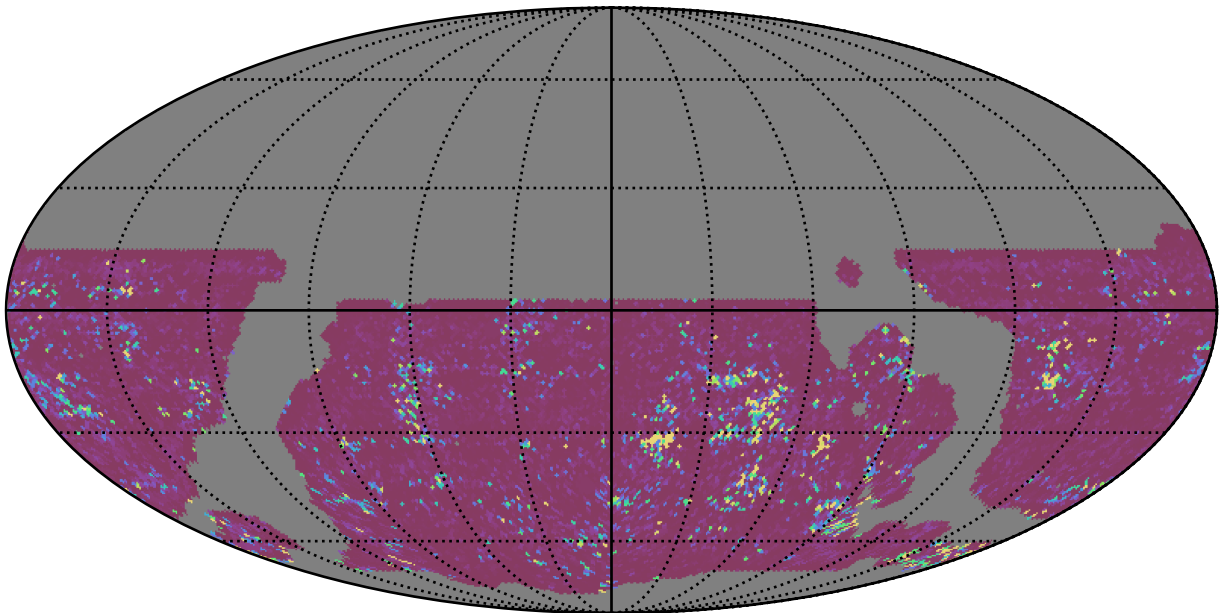
weather_cloudso20v3.4_10yrs WFD u band: 75th Percentile Intranight Timespan
