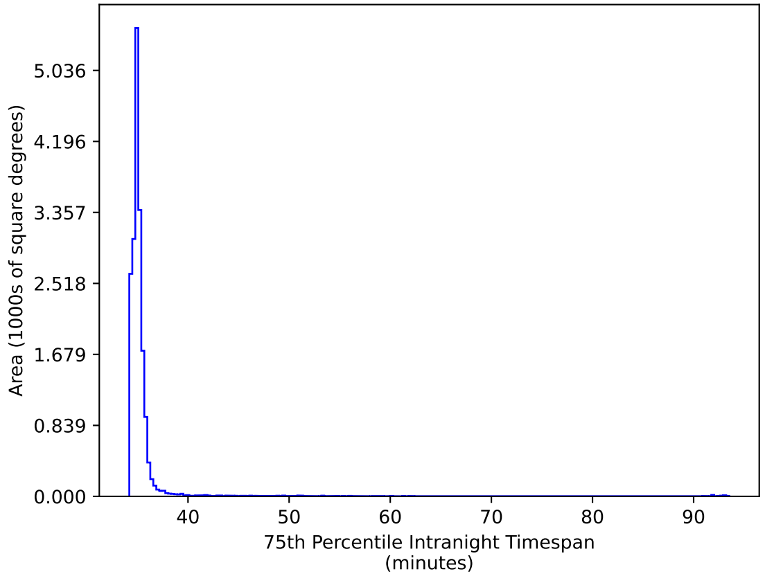
weather_cloudso20v3.4_10yrs WFD ri bands: 75th Percentile Intranight Timespan
