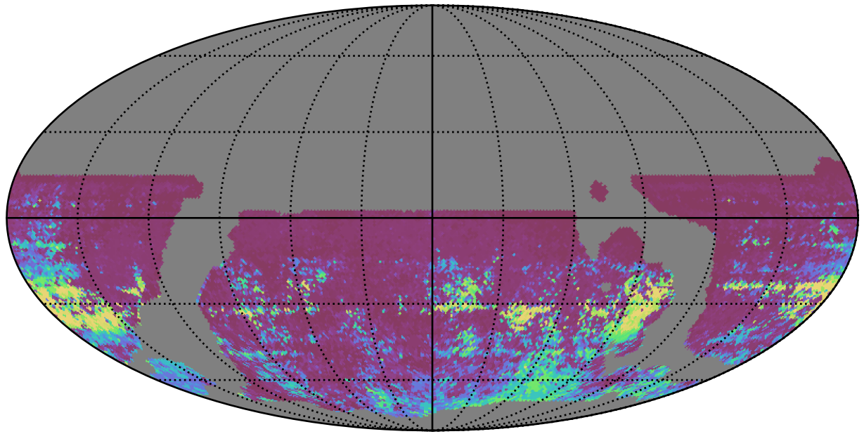
weather_cloudso20v3.4_10yrs WFD r band: 75th Percentile Intranight Timespan
