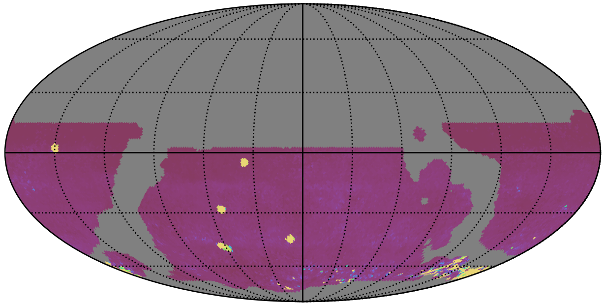
weather_cloudso20v3.4_10yrs WFD iz bands: 75th Percentile Intranight Timespan
