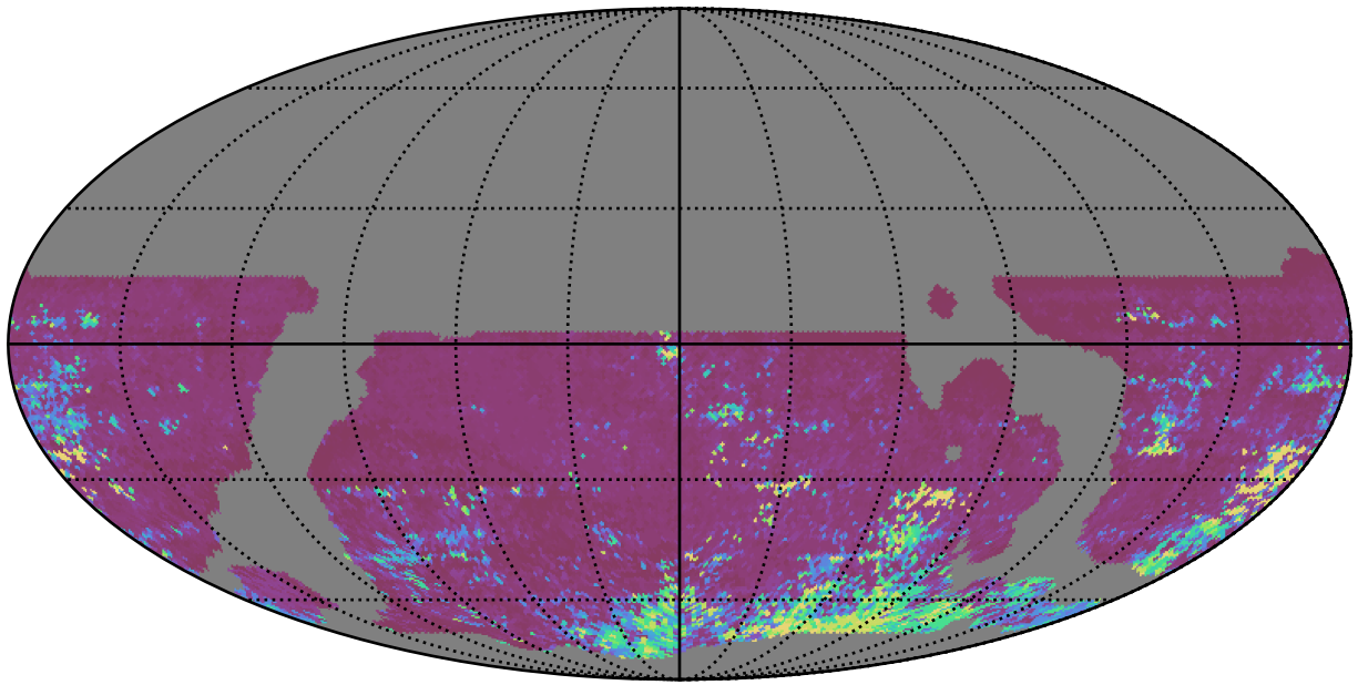
weather_cloudso20v3.4_10yrs WFD i band: 75th Percentile Intranight Timespan
