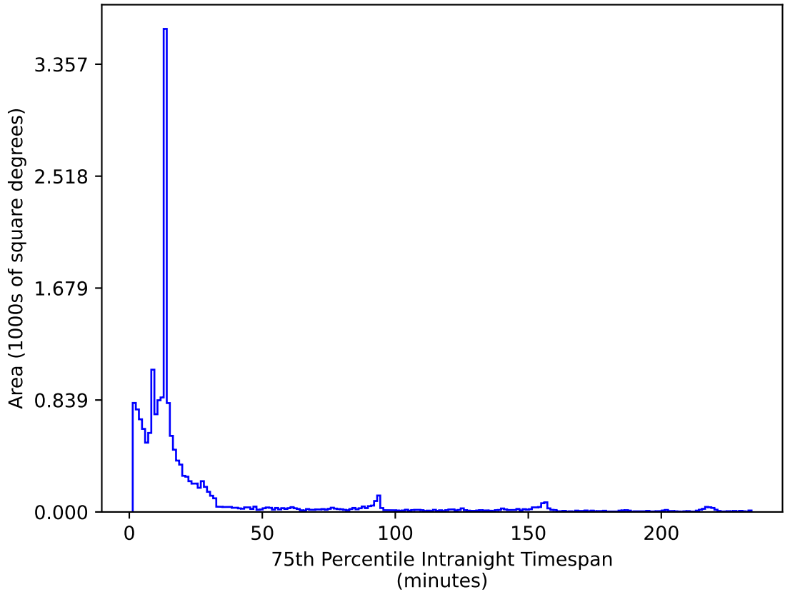
weather_cloudso20v3.4_10yrs WFD i band: 75th Percentile Intranight Timespan
