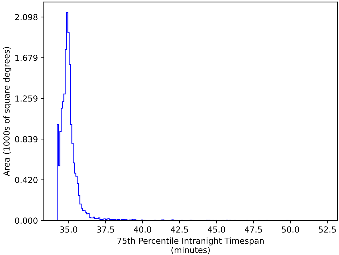
weather_cloudso20v3.4_10yrs WFD gr bands: 75th Percentile Intranight Timespan
