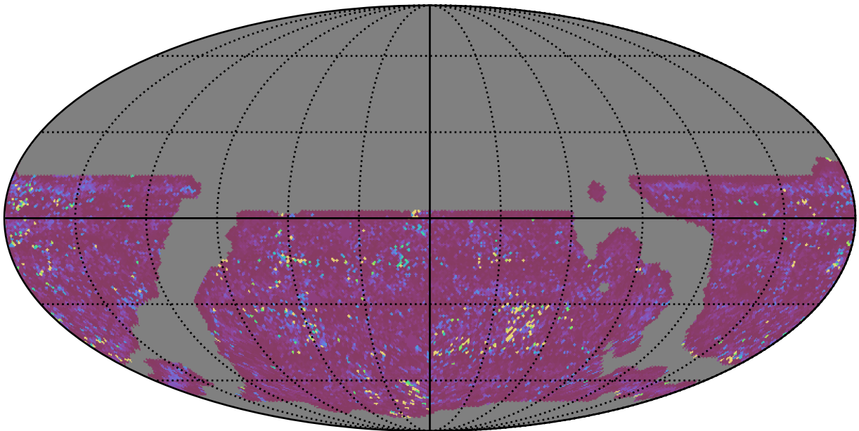
weather_cloudso20v3.4_10yrs WFD g band: 75th Percentile Intranight Timespan
