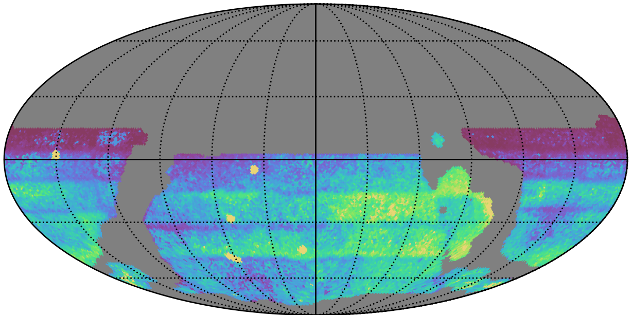
weather_cloudso20v3.4_10yrs WFD all bands: 75th Percentile Intranight Timespan
