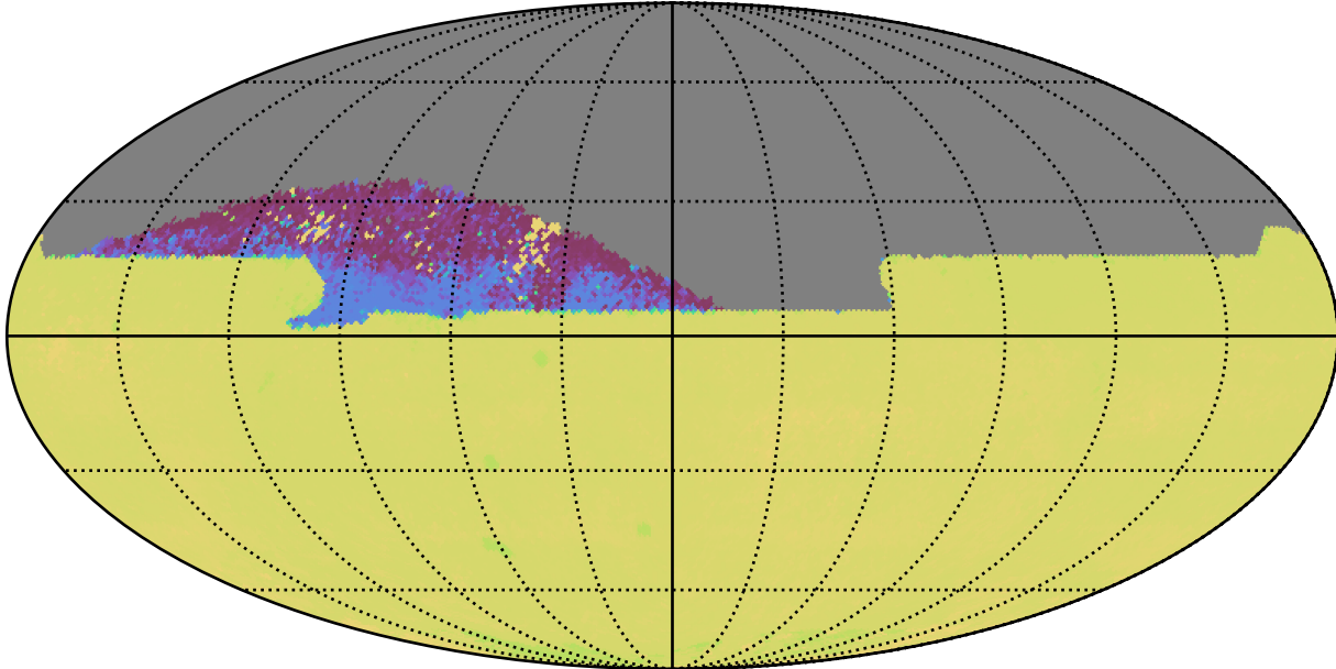
weather_cloudso20v3.4_10yrs All sky zy bands: 75th Percentile Intranight Timespan
