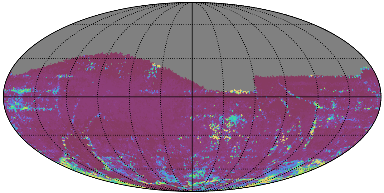
weather_cloudso20v3.4_10yrs All sky z band: 75th Percentile Intranight Timespan
