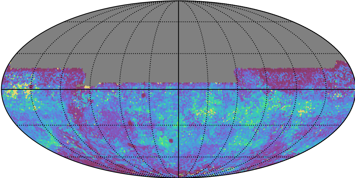
weather_cloudso20v3.4_10yrs All sky y band: 75th Percentile Intranight Timespan
