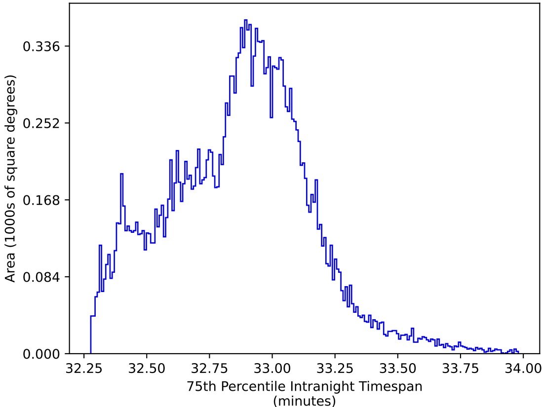
weather_cloudso20v3.4_10yrs All sky y band: 75th Percentile Intranight Timespan
