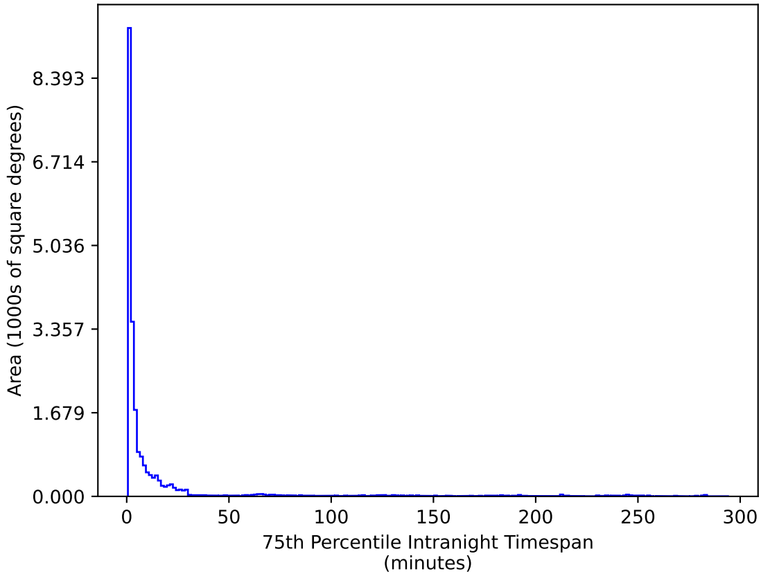
weather_cloudso20v3.4_10yrs All sky u band: 75th Percentile Intranight Timespan
