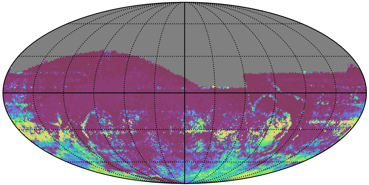
weather_cloudso20v3.4_10yrs All sky r band: 75th Percentile Intranight Timespan
