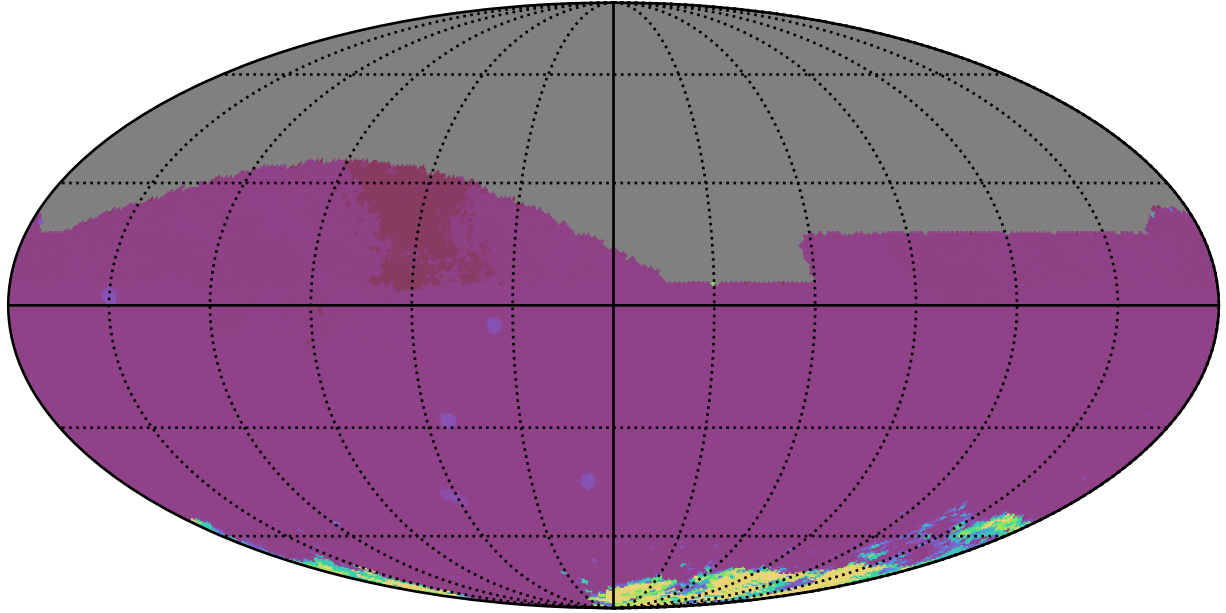
weather_cloudso20v3.4_10yrs All sky iz bands: 75th Percentile Intranight Timespan
