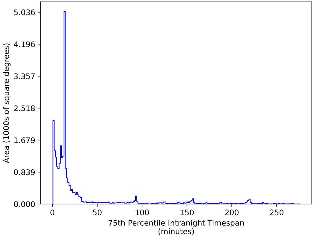
weather_cloudso20v3.4_10yrs All sky i band: 75th Percentile Intranight Timespan
