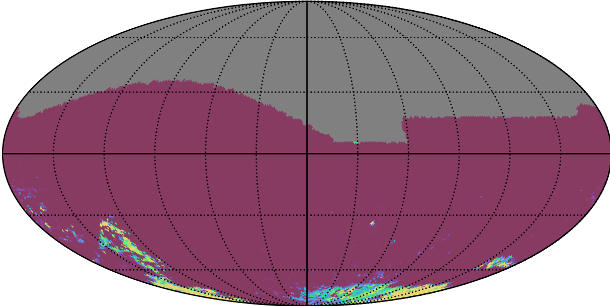
weather_cloudso20v3.4_10yrs All sky gr bands: 75th Percentile Intranight Timespan
