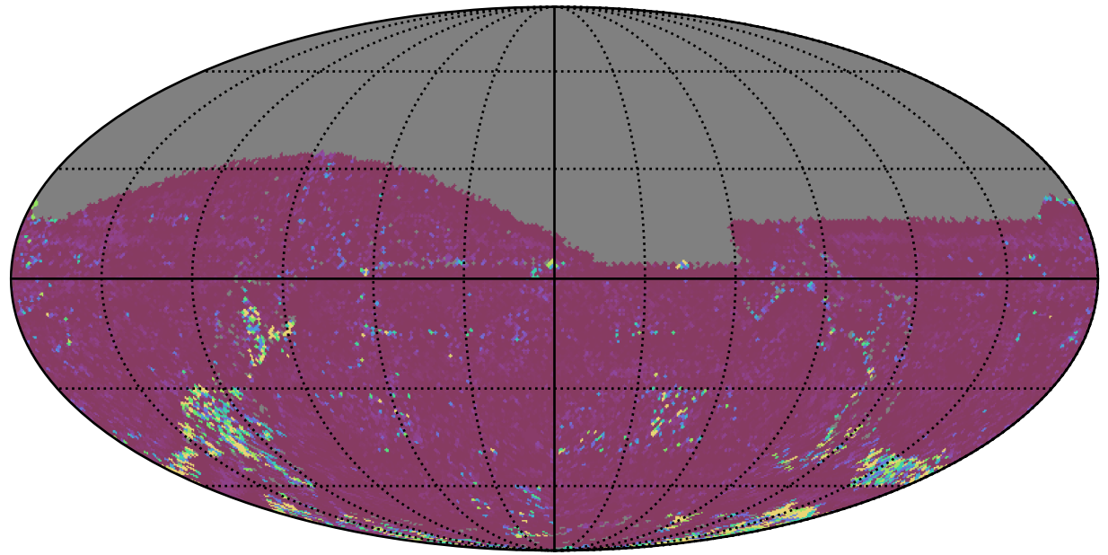
weather_cloudso20v3.4_10yrs All sky g band: 75th Percentile Intranight Timespan
