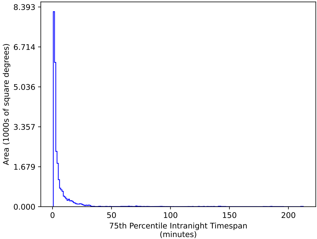
weather_cloudso20v3.4_10yrs All sky g band: 75th Percentile Intranight Timespan
