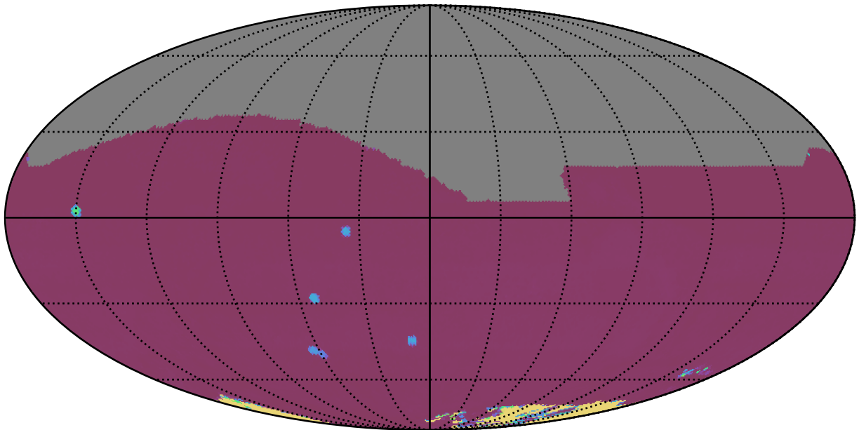
weather_cloudso20v3.4_10yrs All sky all bands: 75th Percentile Intranight Timespan
