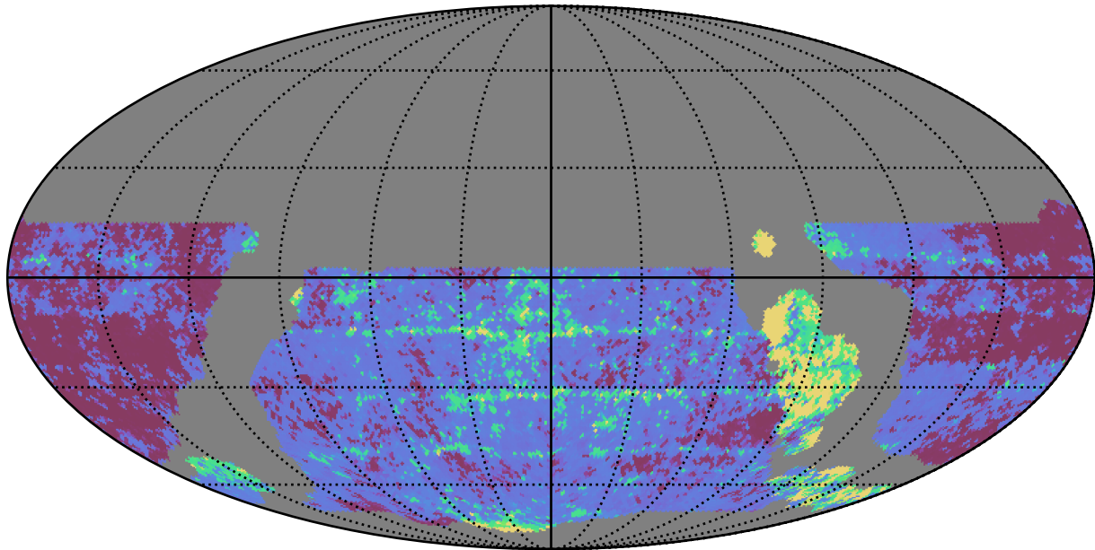
weather_cloudso20v3.4_10yrs WFD y band: 20thPercentile Inter-Night Gap
