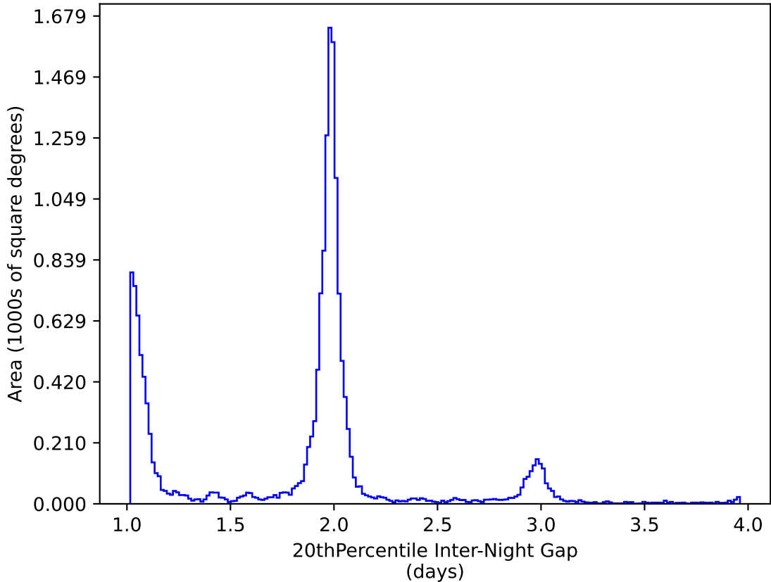
weather_cloudso20v3.4_10yrs WFD y band: 20thPercentile Inter-Night Gap
